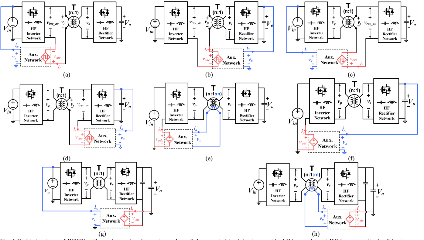
Fig. 6 Eight structures of RDCX with v_{dc} (or v_{cac} ) and v_x series and parallel connected to: (a) primary-side AC bus and input DC bus respectively [20]; (b) primary-side AC bus and output DC bus respectively [20]; (c) secondary-side AC bus and input DC bus respectively; (d) secondary-side AC bus and output DC bus respectively; (e) input DC bus and AC bus respectively [21]-[23], [35]; (f) input DC bus and output DC bus respectively [19]; (g) output DC bus and input DC bus respectively [24], [25]; (h) output DC bus and AC bus respectively [26].
