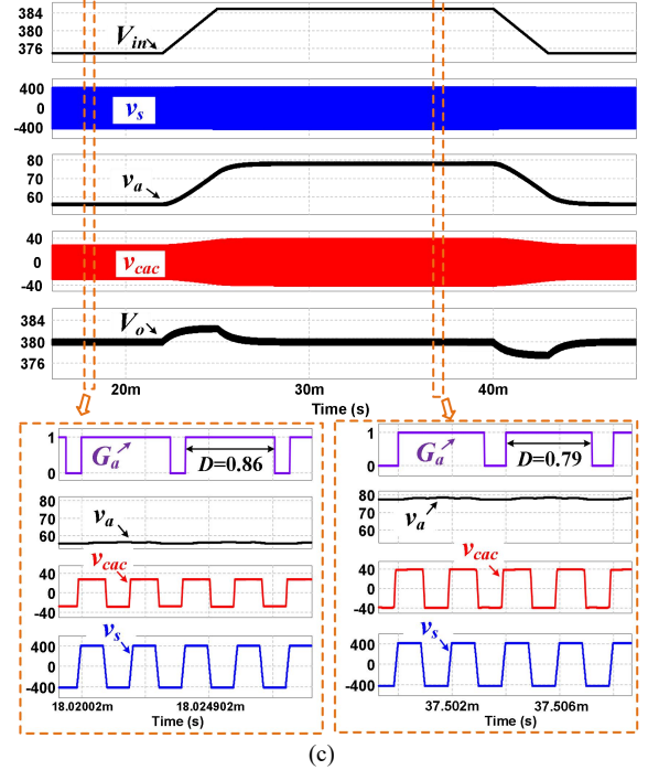
Fig. 9 A 380V/336V RDCX converter based on the structure in Fig. 6(c) with positive v_{cac} : (a) topology; (b) ZVS operation of Q_1 - Q_4 with 380V output and full load; (c) voltage regulation with a step change in V_{in} .
