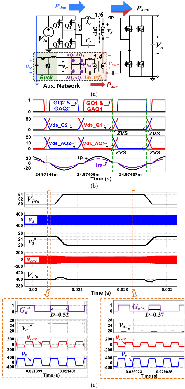
Fig. 10 A 48V/400V RDCX converter based on the structure in Fig. 6(c) with negative v_{cac} : (a) topology; (b) ZVS operation of Q_1 - Q_4 and AQ_1 - AQ_4 at full load; (c) voltage regulation with a step change in V_{in} .
