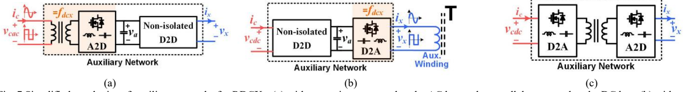
Fig. 7 Simplified topologies of auxiliary networks for RDCXs: (a) with v_{cac} series connected to the AC bus and v_x parallel connected to the DC bus; (b) with v_{dc} series connected to the DC bus and v_x parallel connected to the AC bus; (c) with v_{dc} and v_x connected to the DC buses.
