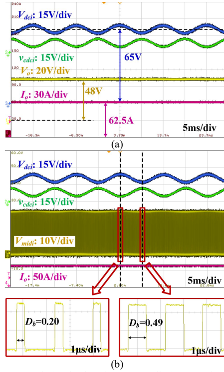
Fig. 16 Voltage regulation in the i th RDCX cell: (a) V_o and v_{cdc} waveforms; (b) v_{cdc} adjustment by varying the duty cycle of Buck D_b .
