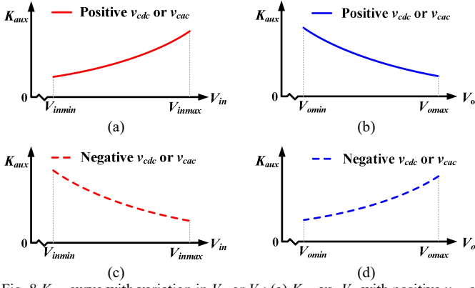
Fig. 8 K_{aux} curve with variation in V_{in} or V_o : (a) K_{aux} vs. V_{in} with positive v_{cdc} or v_{cac} ; (b) K_{aux} vs. V_o with positive v_{cdc} or v_{cac} ; (c) K_{aux} vs. V_{in} with negative v_{cdc} or v_{cac} ; (d) K_{aux} vs. V_o with negative v_{cdc} or v_{cac} .
